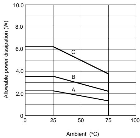
Thermal derating
