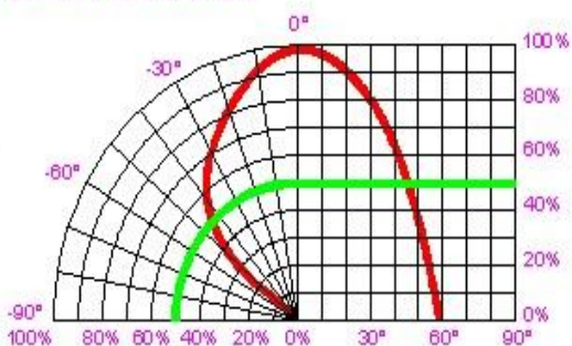
Fig.6 Relative Luminous Intensity vs viewing angle
