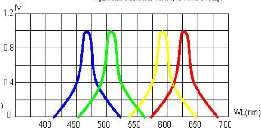
Fig.4 Relative Luminous Intensity vs Wavelength
