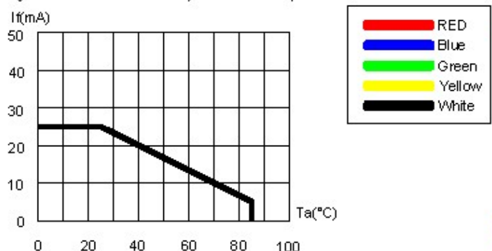
Fig.5 Maximum Forward Current vs Ambient Temperature
