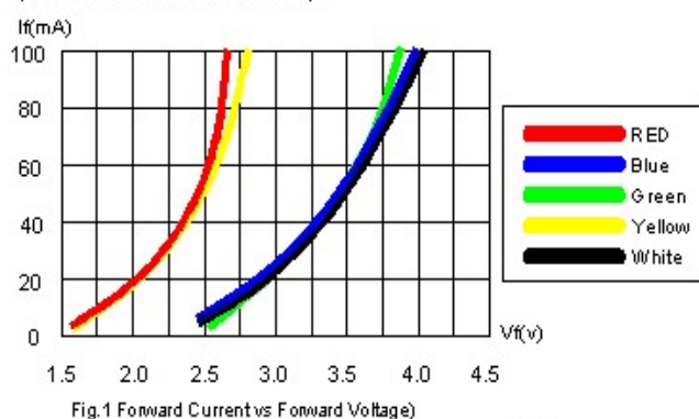
Typical Electrical/Optical Characteristics Curves ( T_a=25^\circ Unless Otherwise Noted)
