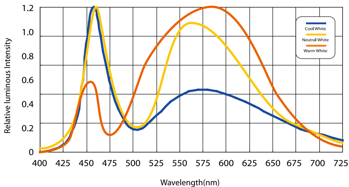
Color Spectrum at a typical CCT for PLCC 3014 0.1W CRI80
