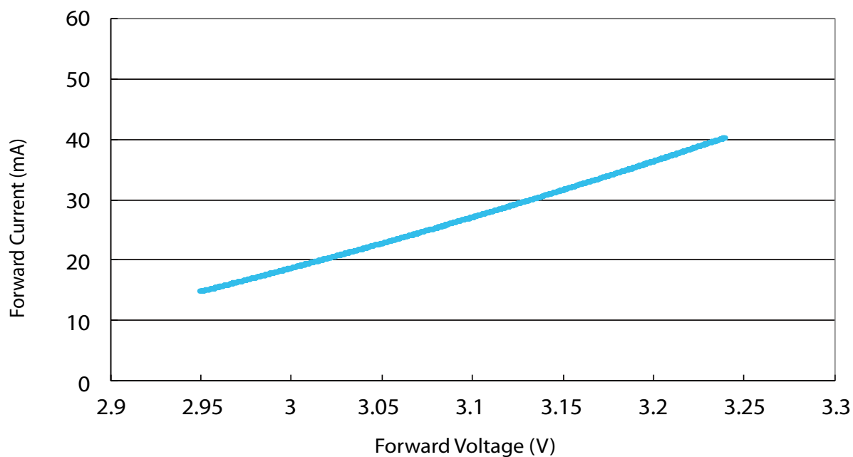
Forward Current vs. Forward Voltage for PLCC 3014 0.1W CRI80
