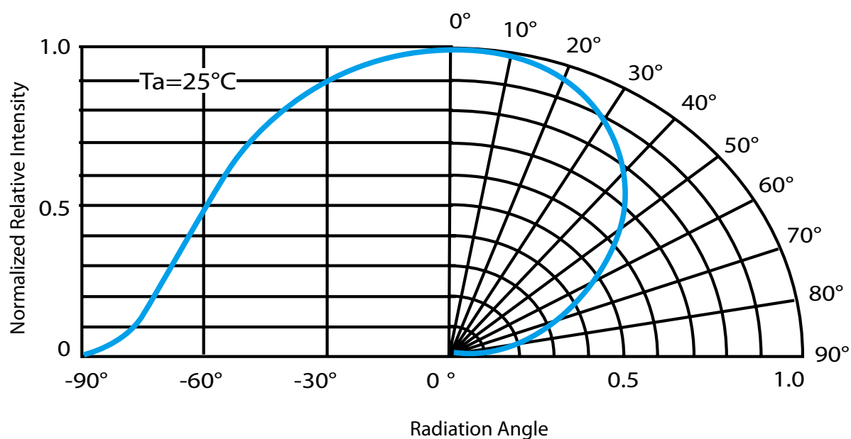
Beam pattern diagram for PLCC 3014 0.1W CRI80
