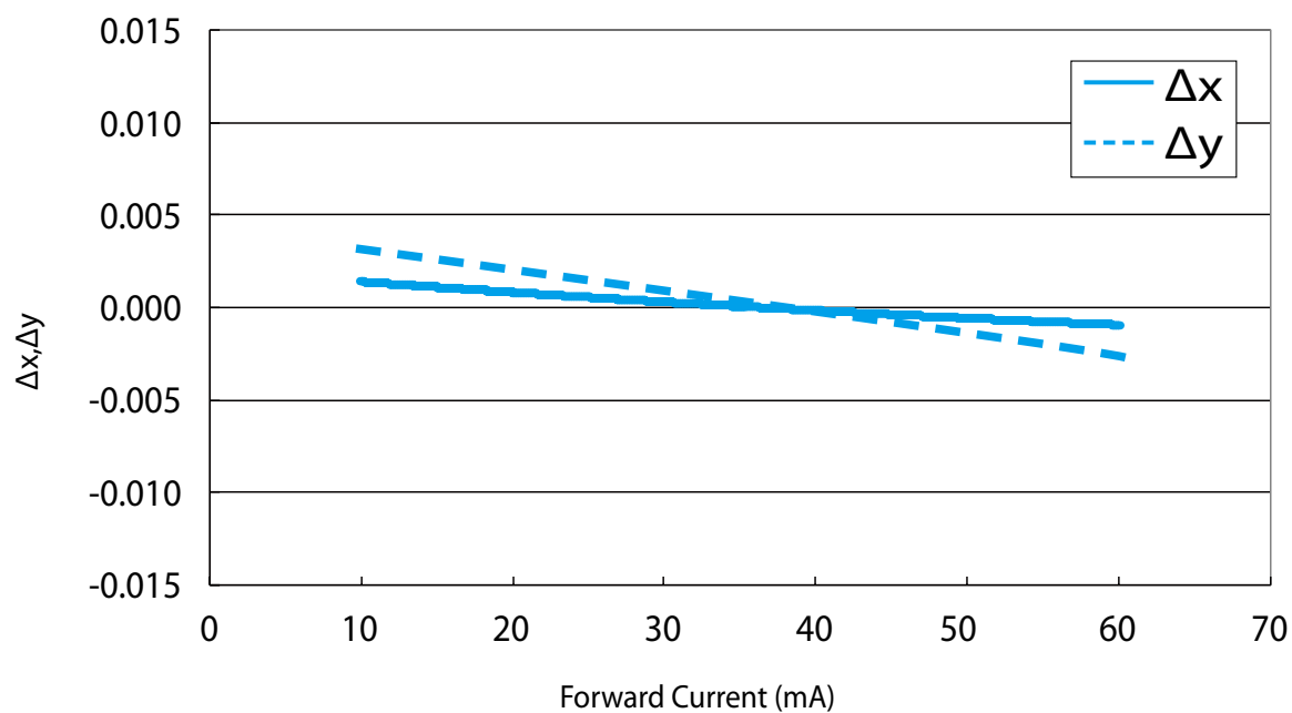
\Delta x, \Delta y vs. Forward Current for PLCC 3014 0.1W CRI80
