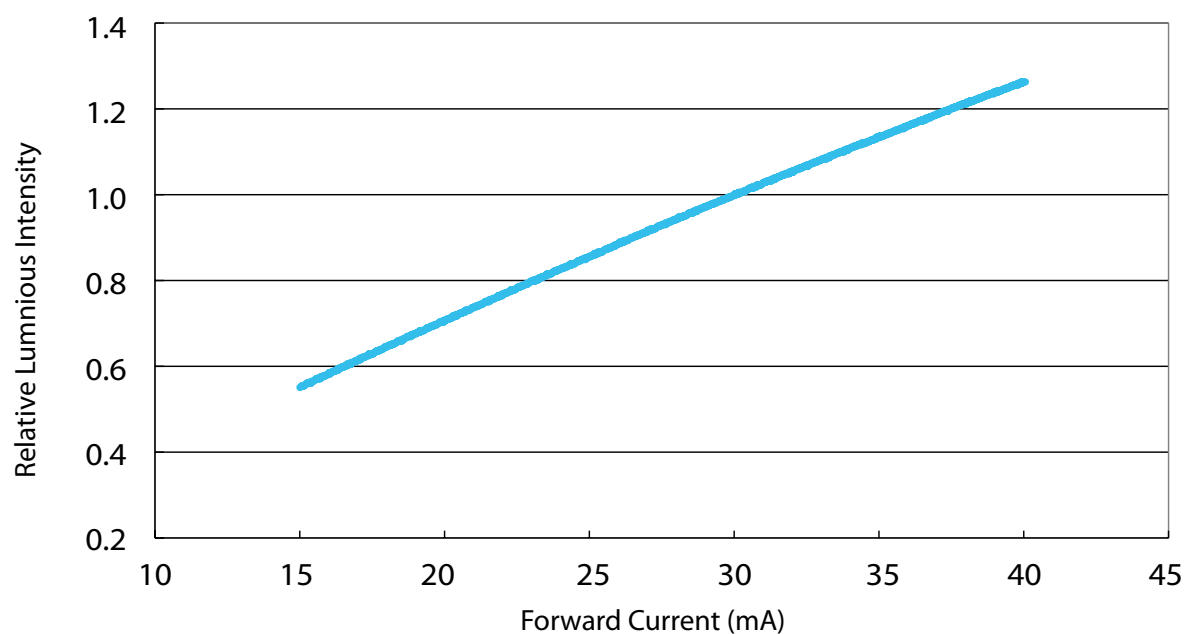
Relative Luminous Intensity vs. Forward Current for PLCC 3014 0.1W CRI80
