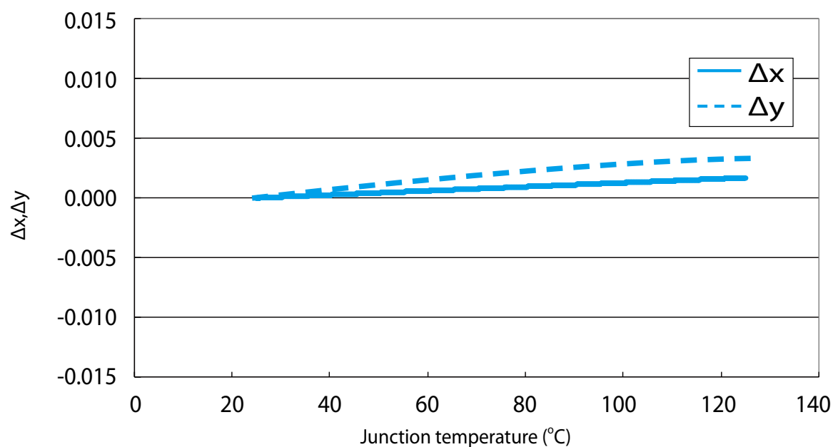
\Delta x, \Delta y vs. Junction temperature for PLCC 3014 0.1W CRI80
