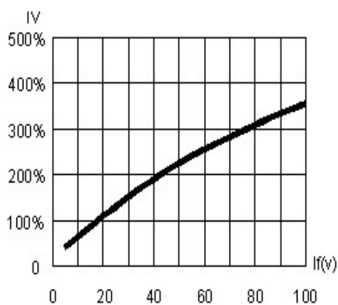
Fig.2 Relative Luminous Intensity vs Forward Voltage
