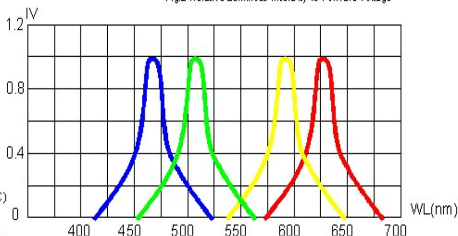
Fig.4 Relative Luminous Intensity vs Wavelength
