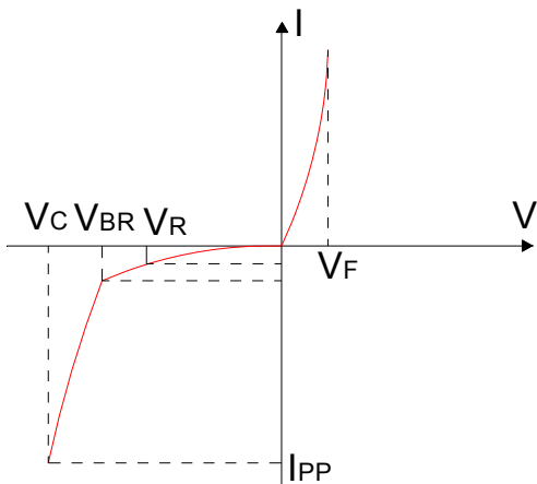
FIG.1:V- I curve characteristics (Uni-directional)
