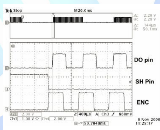
Figure 11. Time to Good Data, External Oscillator, Room Temperature.
