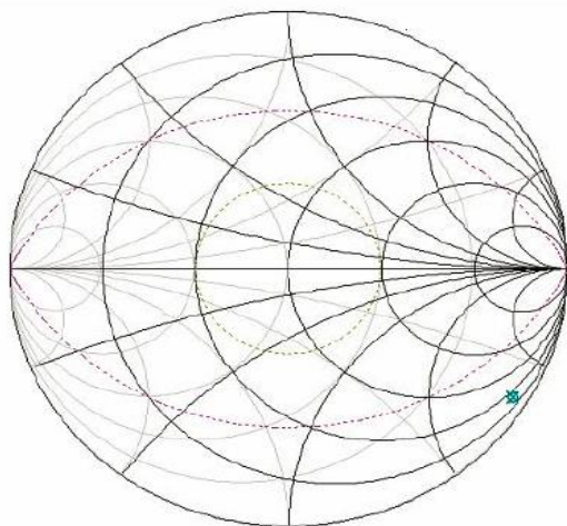
Figure 4: device's input impedance, Z = 18.6 - j174.2\Omega
