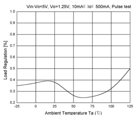
Figure 5. Load Regulation vs. Temperature
