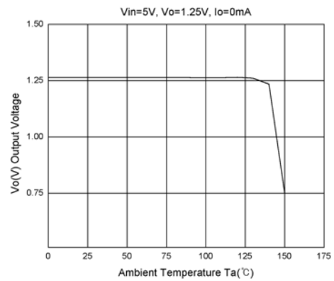
Figure 8. Thermal Shutdown
