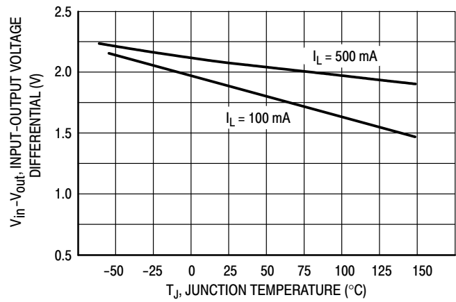
Figure 10. Dropout Voltage
