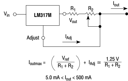
Figure 24. Current Regulator
