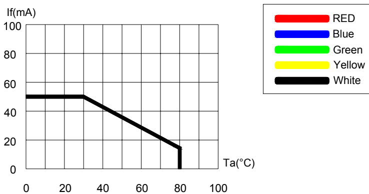
Fig.5 Maximum Forward Current vs Ambient Temperature
