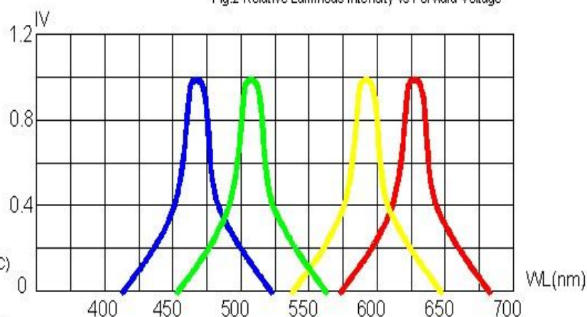
Fig.4 Relative Luminous Intensity vs Wavelength
