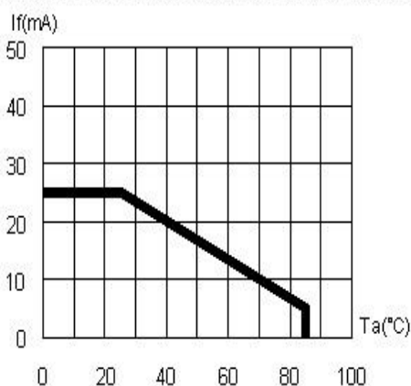
Fig.5 Maximum Forward Current vs Ambient Temperature
