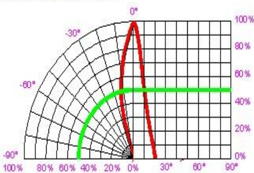
Fig.6 Relative Luminous Intensity vs viewing angle
