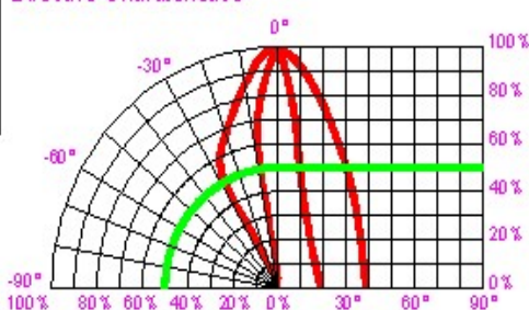
Fig.6 Relative Luminous Intensity vs viewing angle
