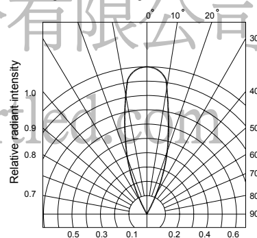
Fig.6 Radiation diagram
