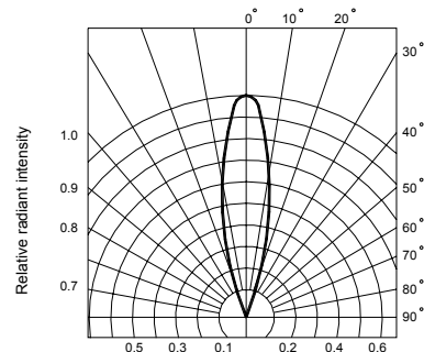
Fig.6 Radiation diagram
