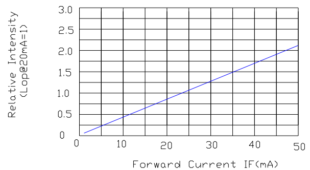
Relative Lumious intensity vs Forward current
