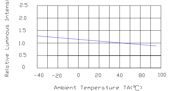
Lumious Intensity Vs. Ambient Temperature
