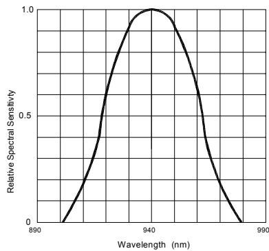
Fig.1 Relative spectral sensitivity vs wavelength
