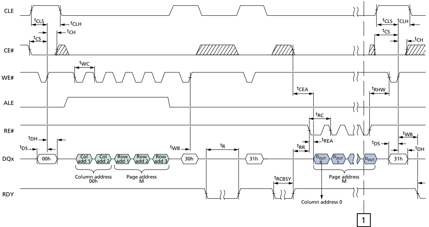
Figure 76: READ PAGE CACHE SEQUENTIAL
