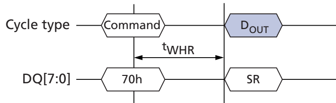
Figure 40: READ STATUS (70h) Operation
