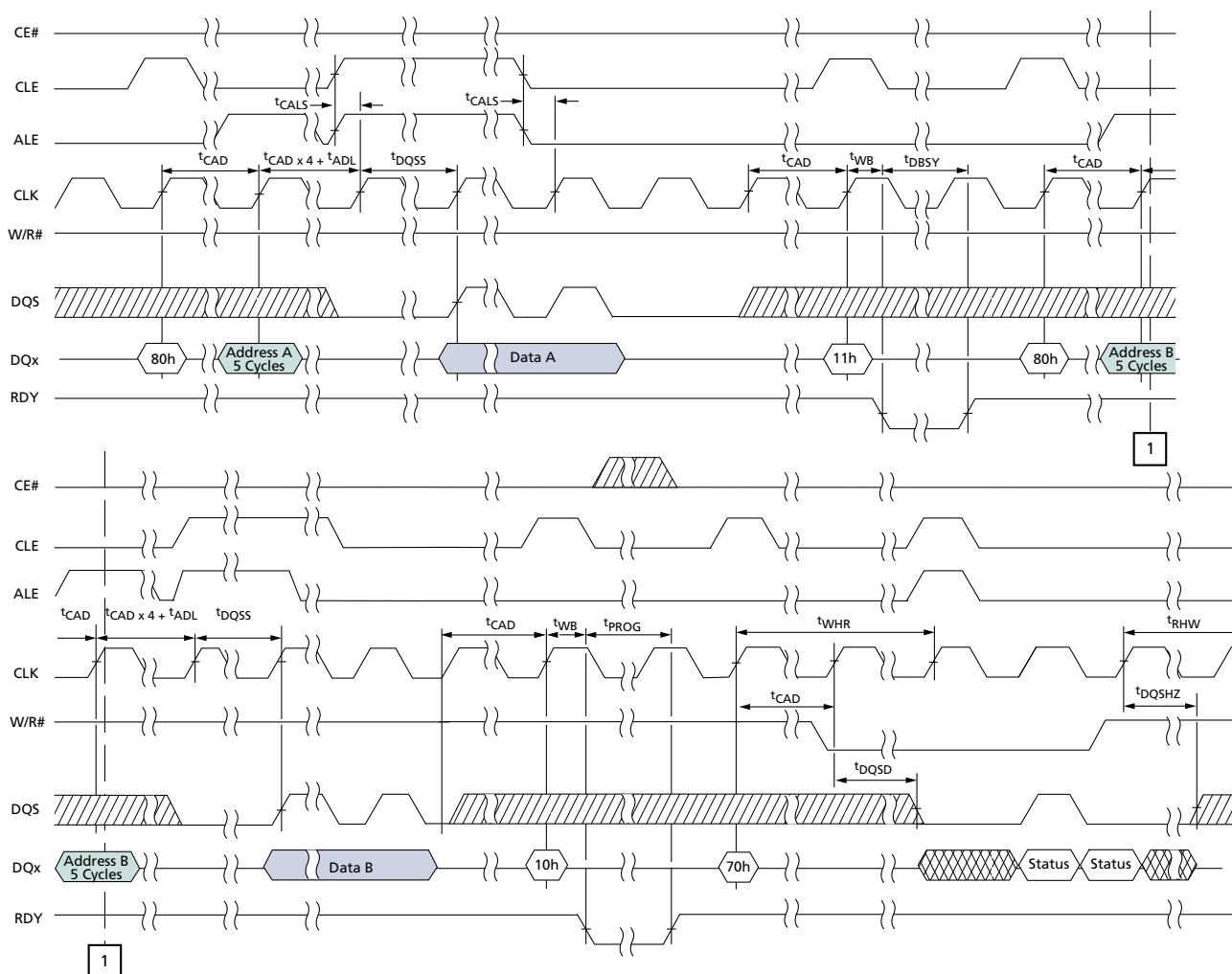
Figure 104: Multi-Plane Program Page
