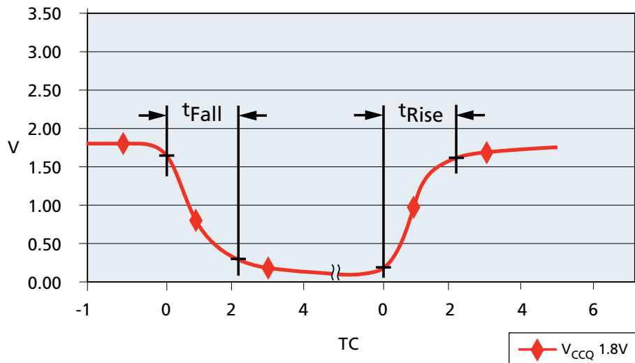
Figure 20: t_{\text{Fall}} and t_{\text{Rise}} ( V_{\text{CCQ}} = 1.7\text{-}1.95\text{V} )
