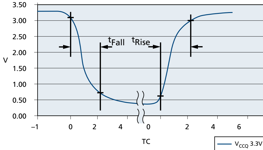
Figure 19: t_{\text{Fall}} and t_{\text{Rise}} ( V_{\text{CCQ}} = 2.7\text{-}3.6\text{V} )
