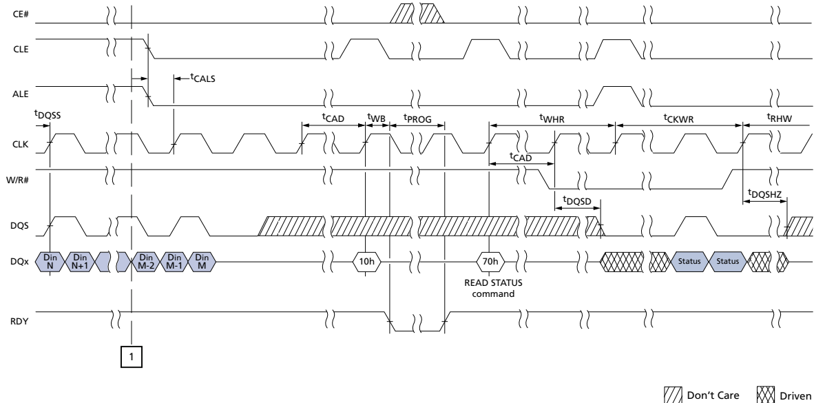
Figure 102: PROGRAM PAGE Operation (2 of 2)
