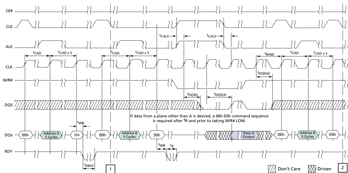
Figure 99: Multi-Plane Read Page (1 of 2)
