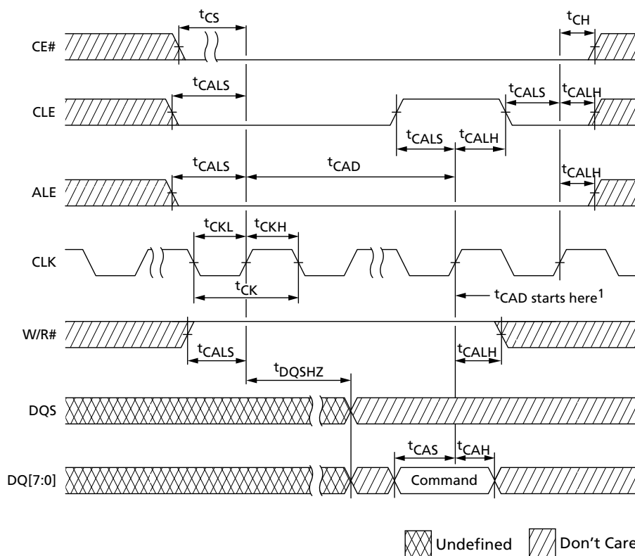
Figure 25: Synchronous Command Cycle
