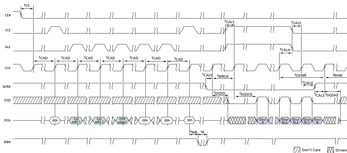
Figure 109: READ OTP PAGE
