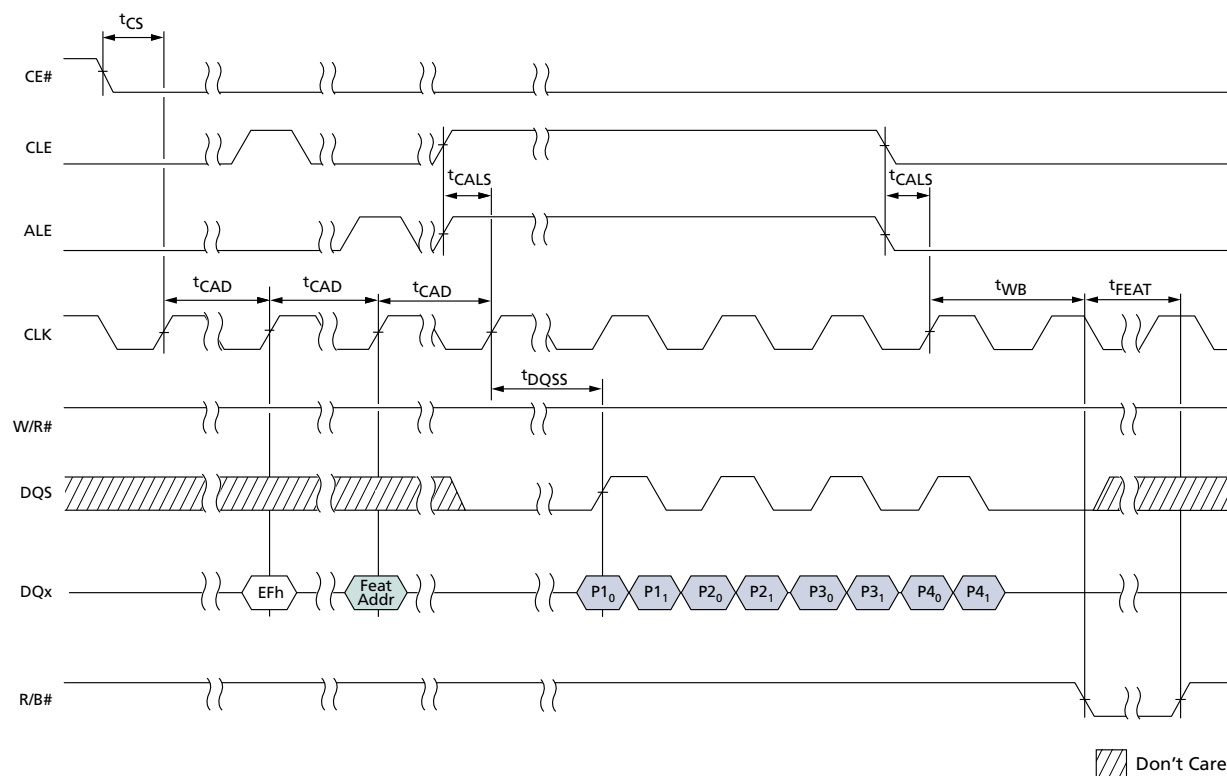
Figure 86: SET FEATURES Operation
