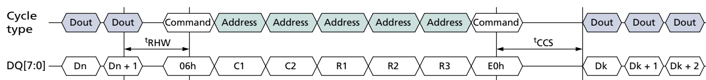
Figure 43: CHANGE READ COLUMN ENHANCED (06h-E0h) Operation
