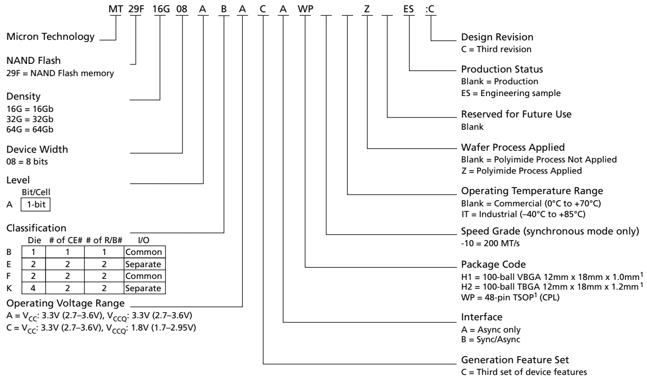
Figure 1: Part Numbering
