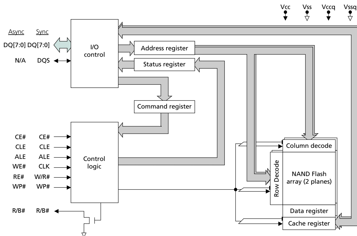
Figure 7: NAND Flash Die (LUN) Functional Block Diagram
