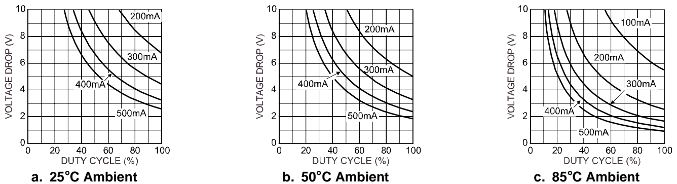
Figure 4. MIC5216-x.xBMM (MSOP-8) on on 1-inch 2 Copper Cladding
