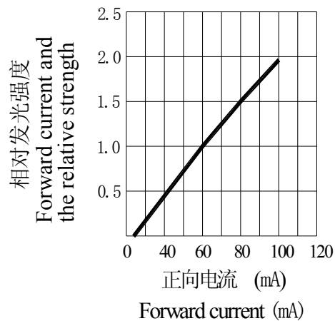
正向电流与相对强度 Forward current and the relative strength
