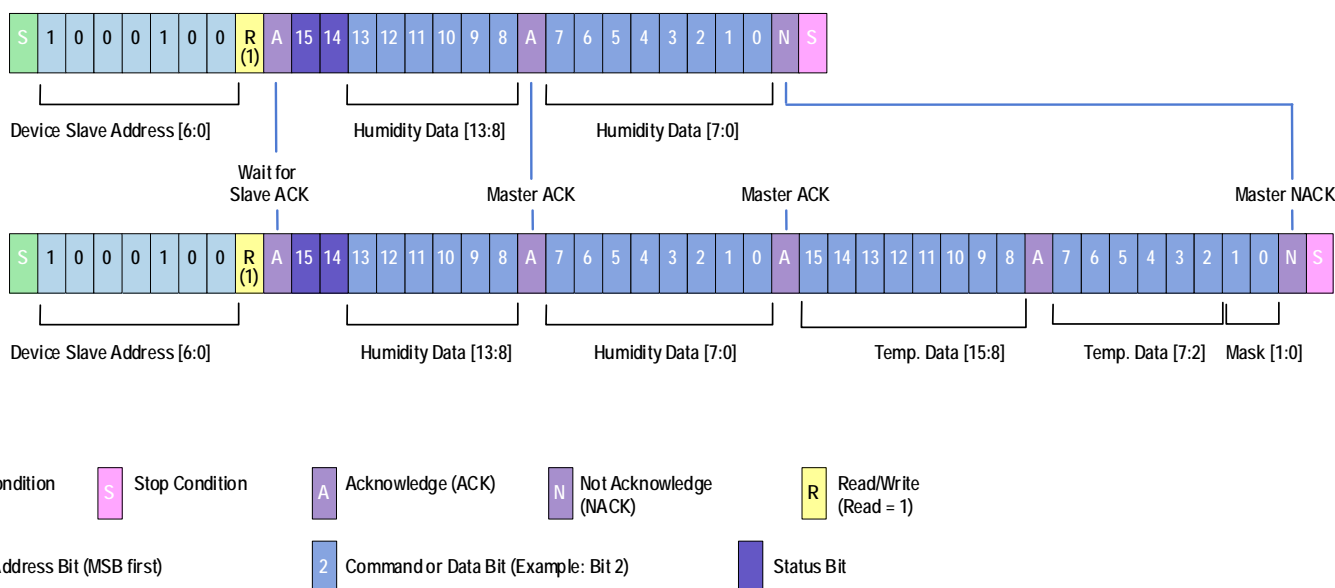
Figure 17. Data Fetch
