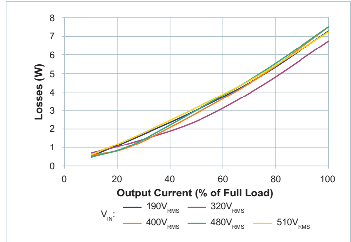
Figure 4 — V_{IN} to V_{OUT} power dissipation vs. V_{IN} (line to line) and I_{OUT} , T_{CASE} = 25^{\circ}\text{C}
