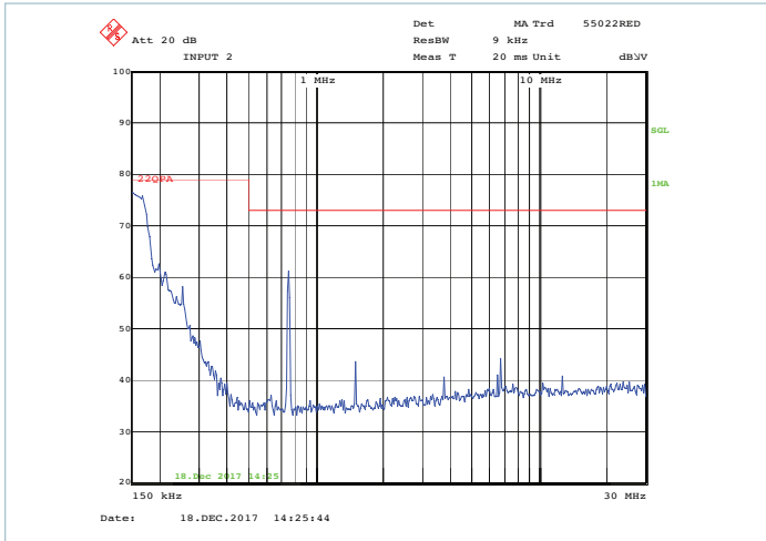
Figure 1 — Typical conducted emissions, peak scan, with BCM4414VG0F4440T02 VIA, 400V AC 90% load, no external components
