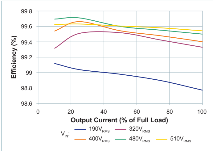
Figure 3 — V_{IN} to V_{OUT} efficiency vs. V_{IN} (line to line) and I_{OUT} , T_{CASE} = 25^{\circ}\text{C}
