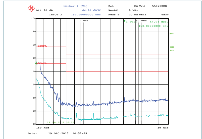
Figure 2 — Typical conducted emissions, peak and average scan, with BCM4414VG0F4440T02 VIA, 400V AC 90% load, with external components as shown in typical application on page 3
