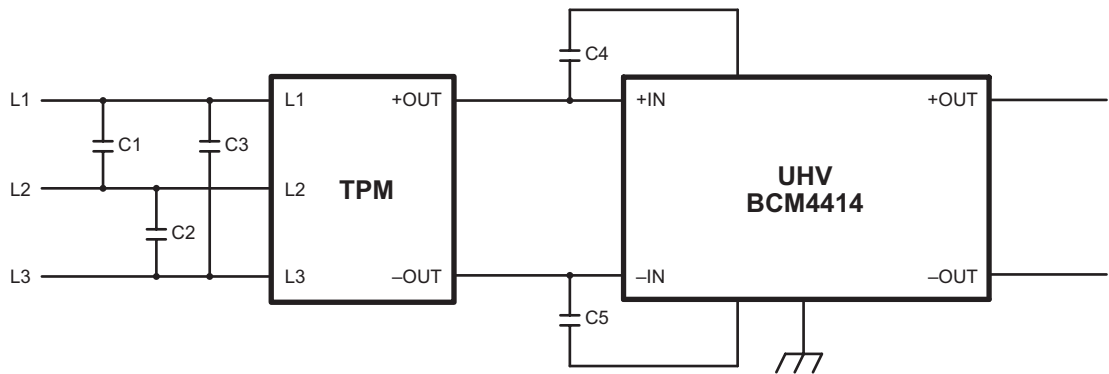
Typical Application: TPM configuration and external components used for conducted-emission scan shown in Figure 2
