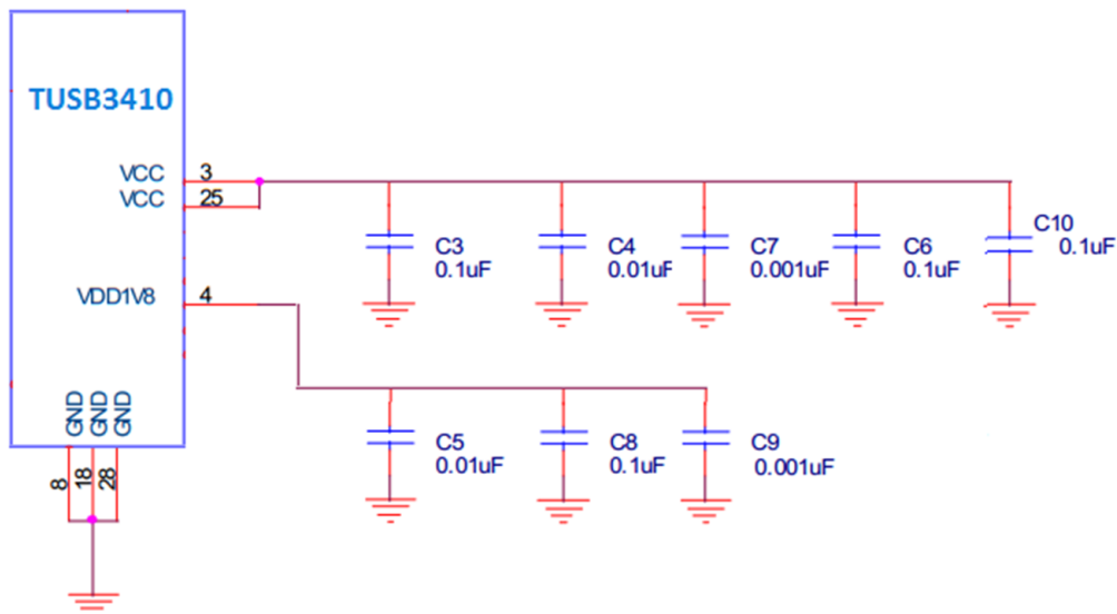
Figure 6-6. Power Implementation
