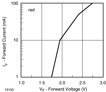
Fig. 32 - Forward Current vs. Forward Voltage
