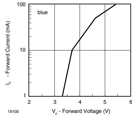
Fig. 12 - Forward Current vs. Forward Voltage
