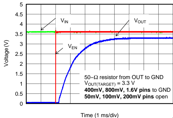
Figure 36. EN Pulse On Response (Over Stable V_{IN} )
