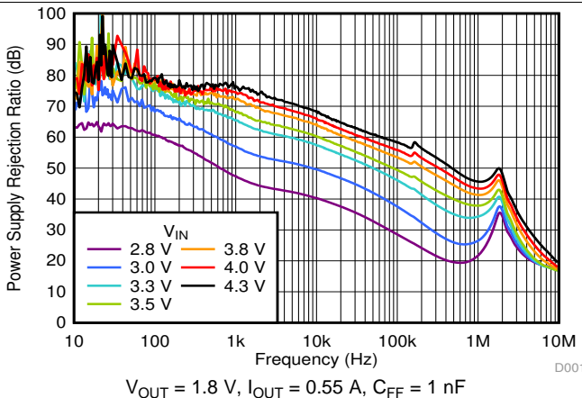
Figure 27. PSRR vs V_{IN}
