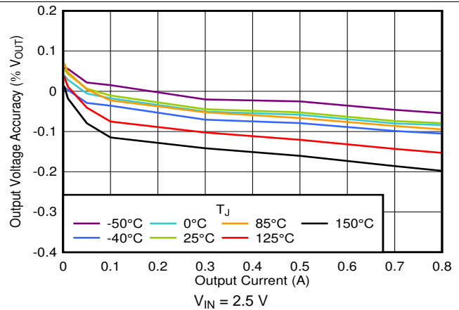
Figure 2. V_{OUT} Accuracy vs I_{OUT}
