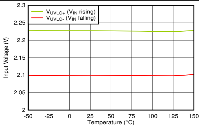
Figure 25. UVLO Thresholds vs Temperature
