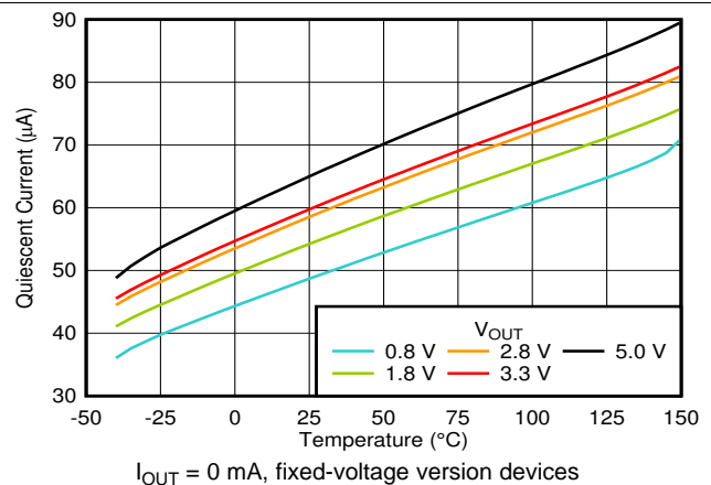
Figure 6. I_Q vs Temperature
