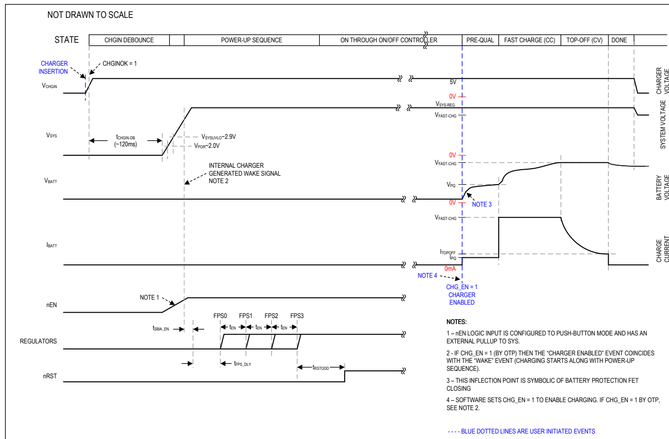
Figure 11. Startup Timing Diagram Due to Charge Source Insertion
