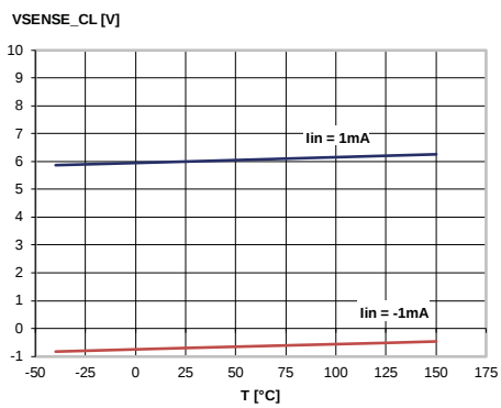
Figure 28: Vsense clamp vs. Tcase
