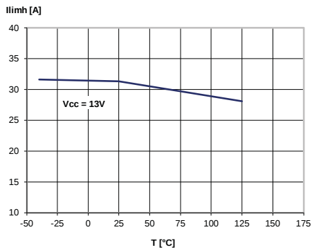
Figure 26: IlimH vs. Tcase
