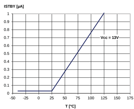
Figure 11: Standby current
