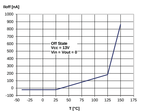
Figure 10: OFF-state output current
