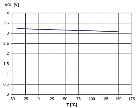
Figure 27: OFF-state open-load voltage detection threshold
