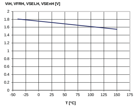
Figure 13: Logic Input high level voltage
