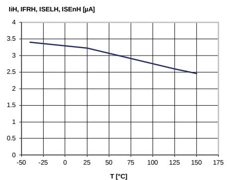
Figure 15: High level logic input current
