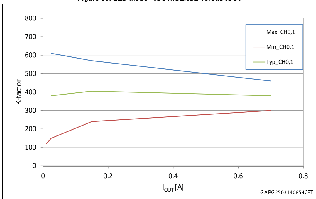
Figure 31: LED Mode - current sense precision vs. I_{OUT}
