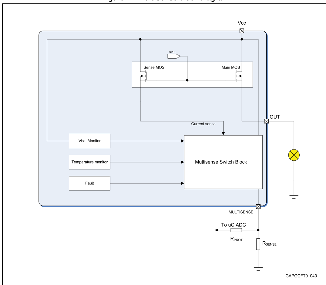
Figure 42: MultiSense block diagram
