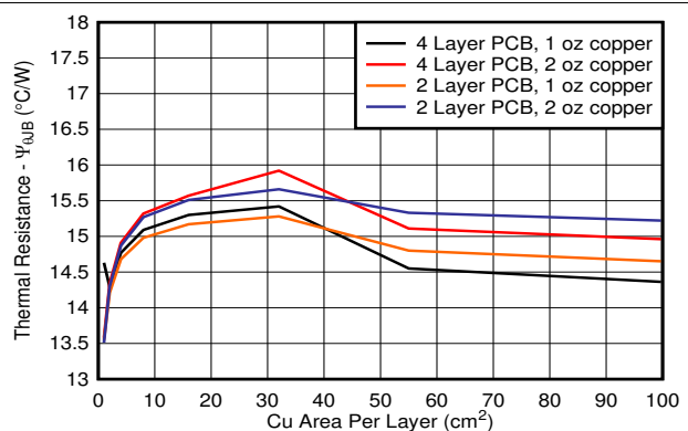
Figure 8-5. \psi_{JB} vs Copper Area 2s2p DCY Package
