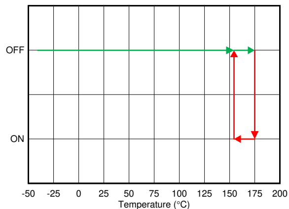
Figure 6-32. Thermal Shutdown
