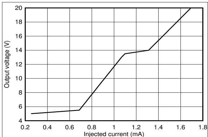
Figure 6-31. Output Voltage vs Injected Current
