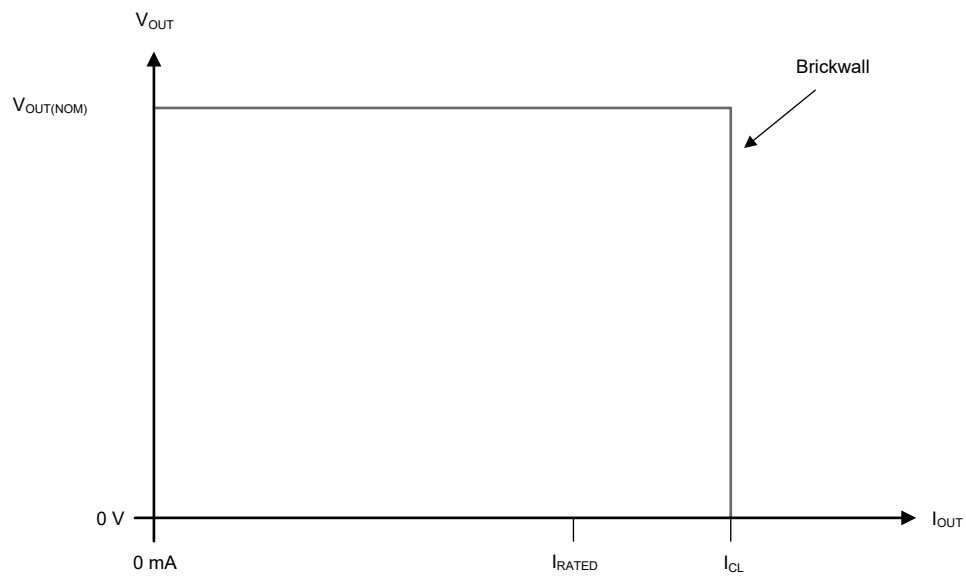
Figure 7-3. Current Limit
