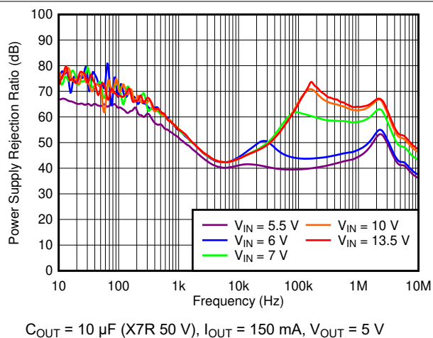
Figure 6-10. PSRR vs Frequency and V_{IN}
