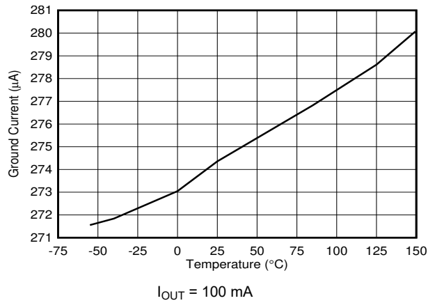
Figure 6-25. Ground Current
