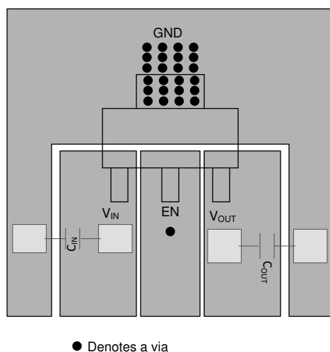
Figure 10-1. SOT-223 (DCY) Layout
