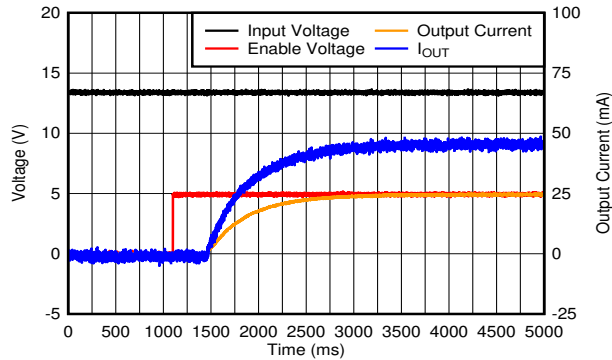
Figure 8-8. Power-Up Waveform
