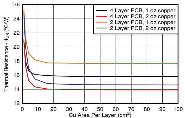
Figure 8-3. \psi_{JB} vs Copper Area 2s2p DRB Package
