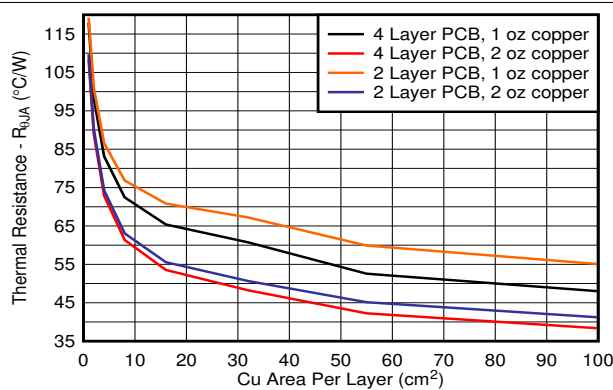
Figure 8-4. R_{\theta JA} vs Copper Area 2s2p DCY Package
