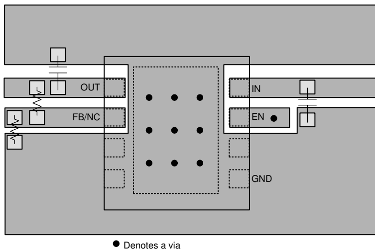
Figure 10-2. VSON (DRB) Layout
