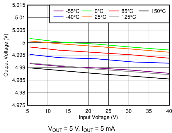
Figure 6-3. Line Regulation vs V_{IN}
