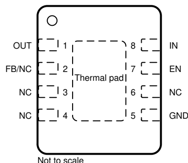
Figure 5-2. DRB Package, 8-Pin VSON, Top View
