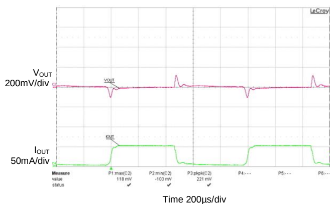
Load Transient C_{IN}=1\mu\text{F} , C_{OUT}=1\mu\text{F} , V_{IN}=V_{OUT}+1.5\text{V} to 30\text{V} , I_{OUT}=0 to 50\text{mA}
