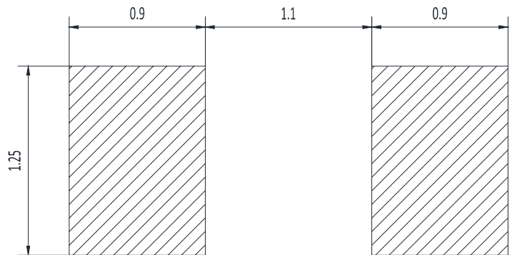
推荐焊盘尺寸 Recommend Soldering Pad
