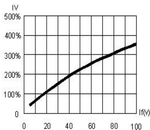
Fig.2 Relative Luminous Intensity vs Forward Voltage
