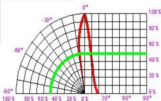
Fig.6 Relative Luminous Intensity vs viewing angle
