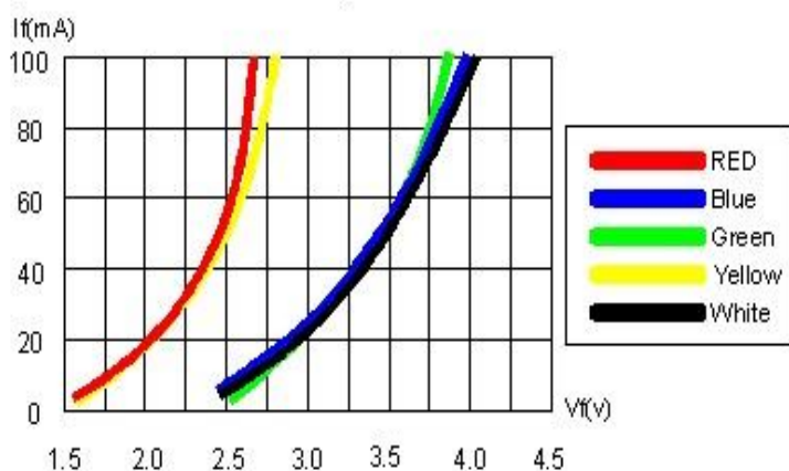
Fig.1 Forward Current vs Forward Voltage)
