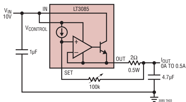
Current Source
